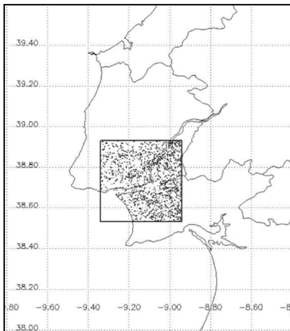
Fig. 1 – AED occurrence area considered in order to define sample days during autumn in Lisbon (2003-2009). The dots indicate the locations of EAD observed in the sample (except for the maritime area of the rectangle).
